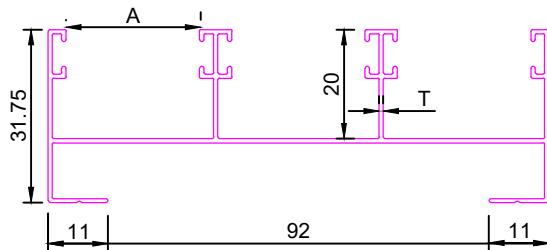
3/4" 3 TRACK TOP
