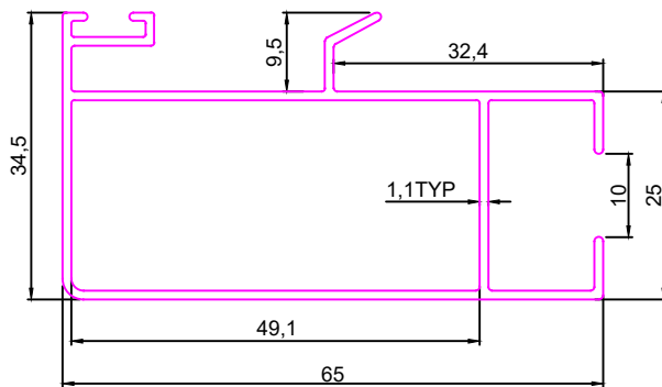
SEC No. 8931
