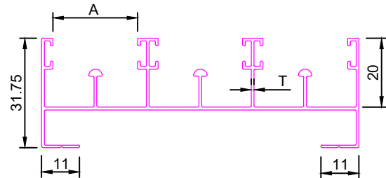
3/4" 3 TRACK BOTTOM
