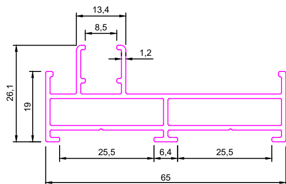
SEC No. 8932
