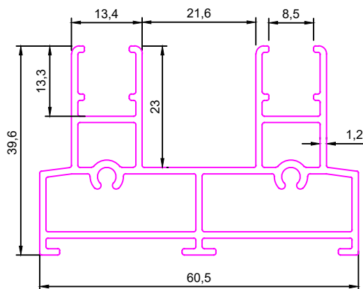
SEC No. 8931
