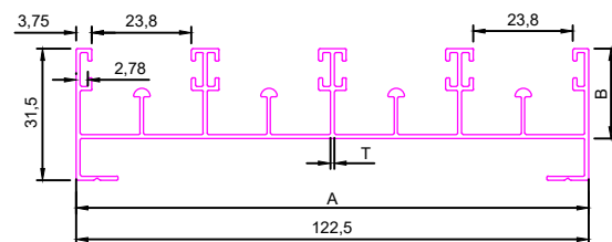
3/4" 4 TRACK BOTTOM
