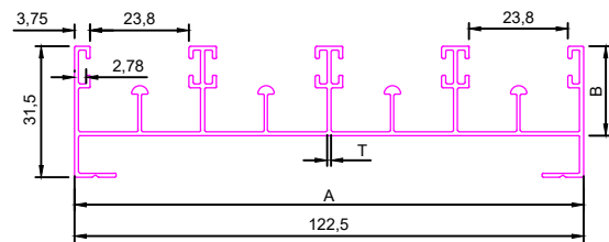
3/4" 4 TRACK BOTTOM
