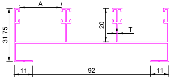
3/4" 3 TRACK TOP
