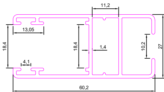
27x60 Shutter
