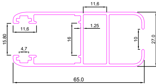
Euro Shutter
